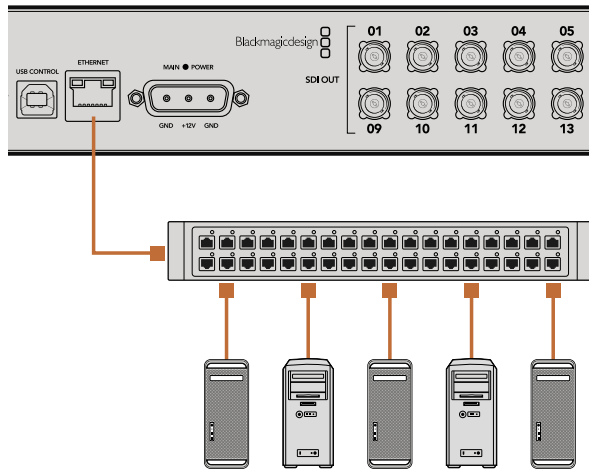
Micro Videohub connecting to an Ethernet Network.
