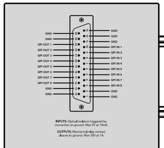
Pinout diagram of the DB25 connector
