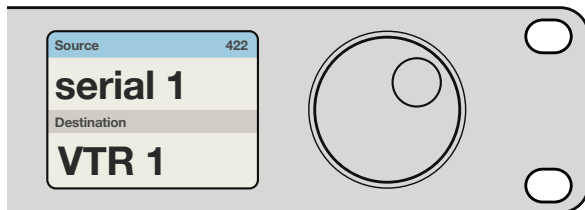
Choose the 422 routing level if you want to see all equipment with RS-422 remote deck control, including equipment with mismatched labels and also remote controllers. In this example, the capture card (Edit 1) has a mismatched label for its remote port (serial 1) and is only listed when the routing level is set to 422.
