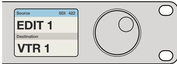
Choose the SDI 422 routing level if you only want to see SDI video equipment with RS-422 deck control. In this example, the capture card (Edit 1) and the deck (VTR 1) are listed because they both have SDI and RS-422 ports.
