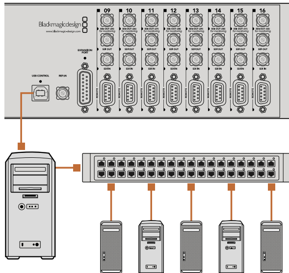
Studio Videohub connecting to a server via USB.
